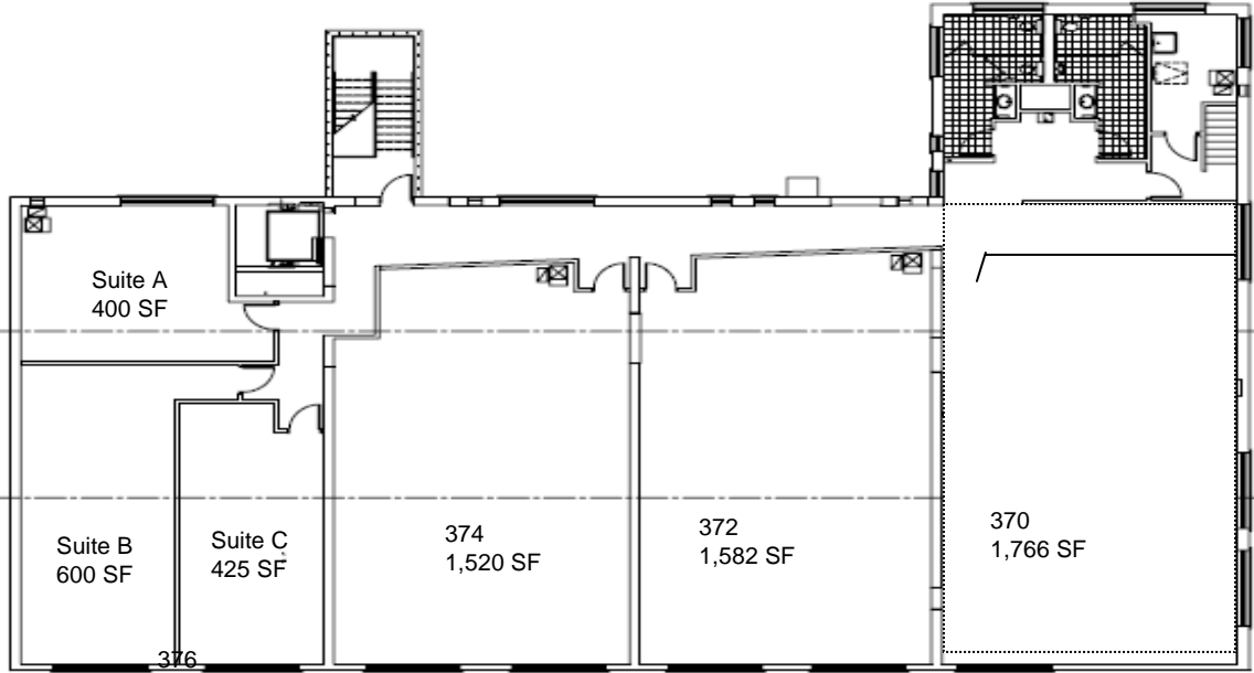
1 st Floor
